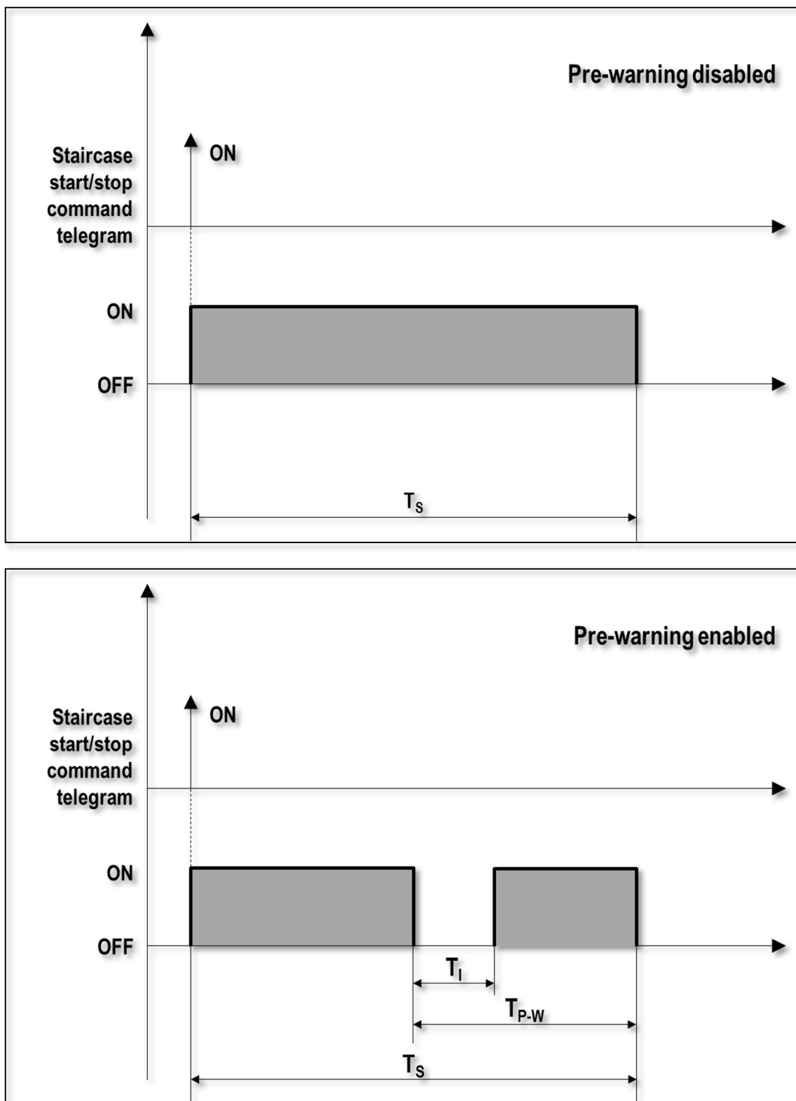
Fig. 6 - Pre-warning feature
