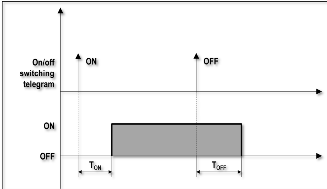
Fig. 3 - Time delay
