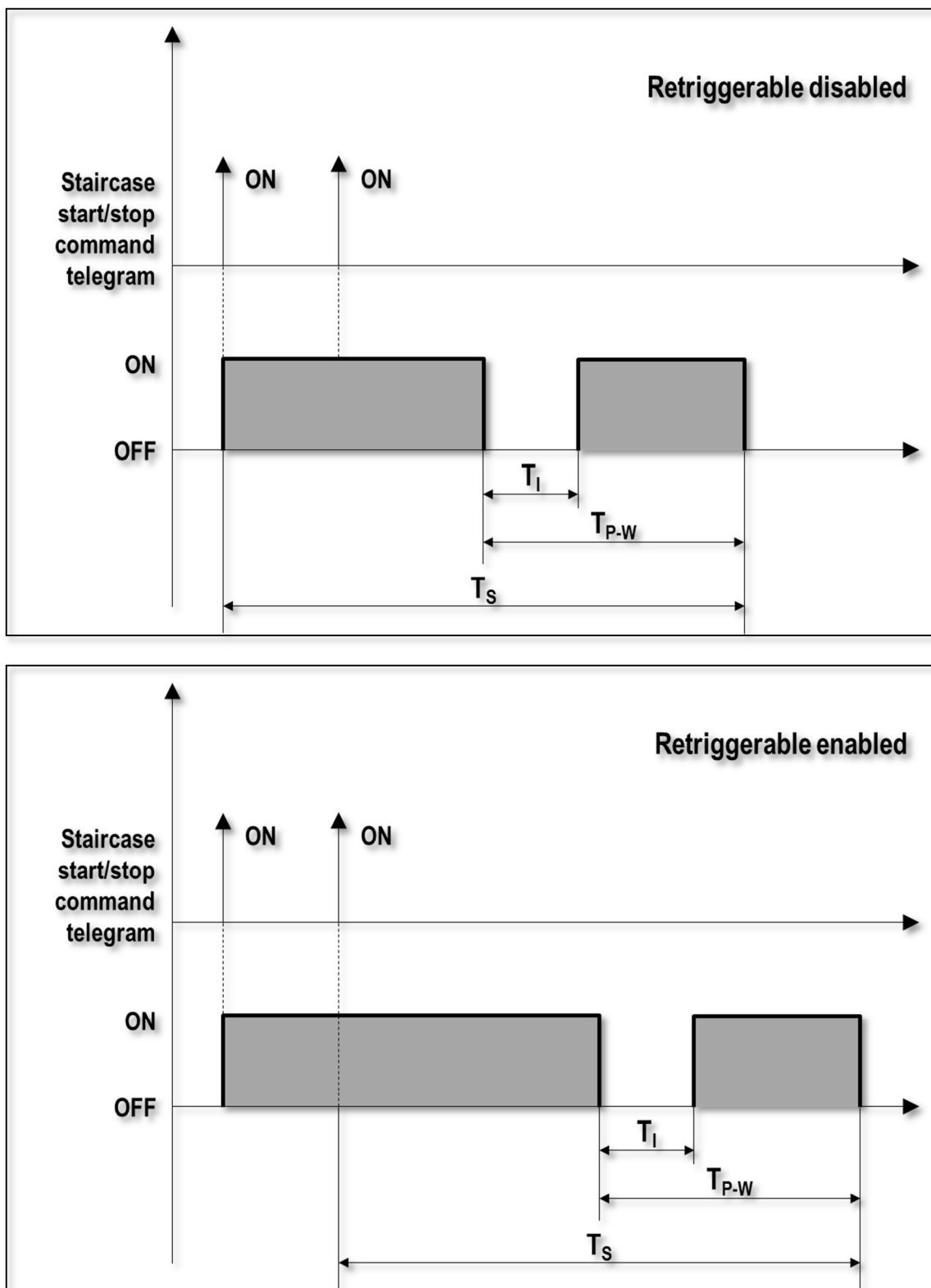
Fig. 5 - Retrigger feature
