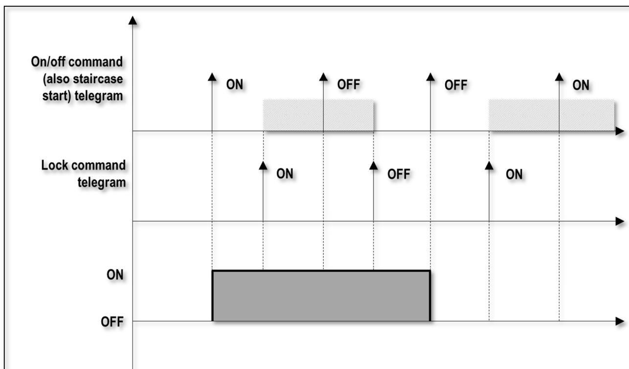
Fig. 11 - Lock function
