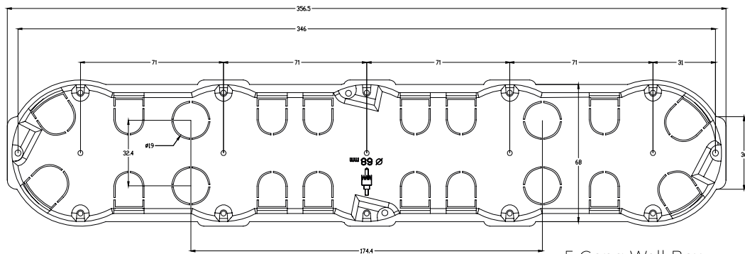
5 Gang Wall Box
