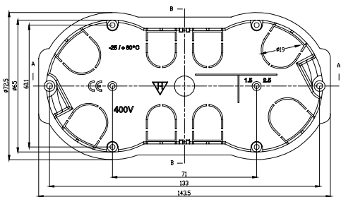
2 Gang Wall Box
