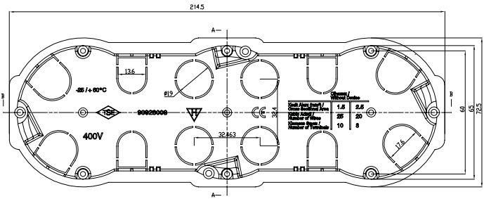
3 Gang Wall Box
