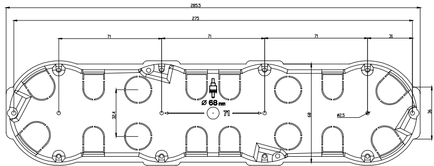
4 Gang Wall Box
