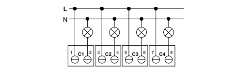
e Connection loads EK-FA1-TP (4-fold)
