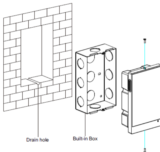
Fig. 1 : Connection Diagram of ITR640-0001 Outdoor Intercom Unit
