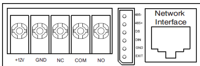
Fig. 8 : Connectors of the ITR640-0001
