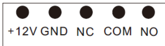
Fig. 10 : Power input connections
