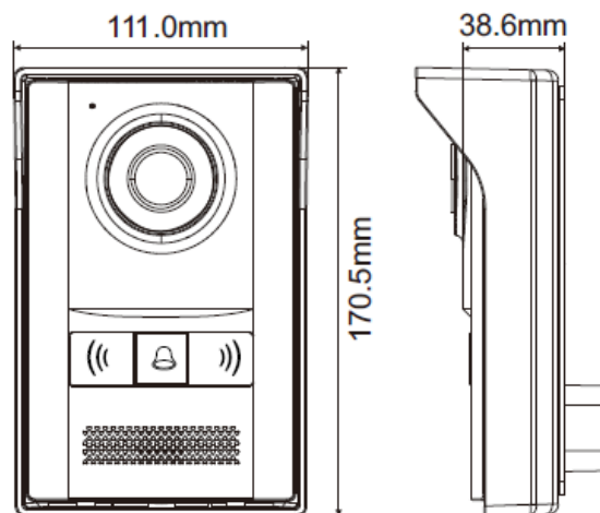
Fig. 3 : Dimension Diagram of ITR640-0001 Outdoor Intercom Unit
