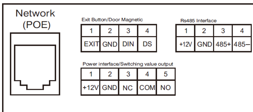
Fig. 9 : Connectors of the ITR641-0001
