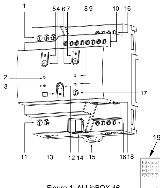
Figure 1: ALLinBOX 46
