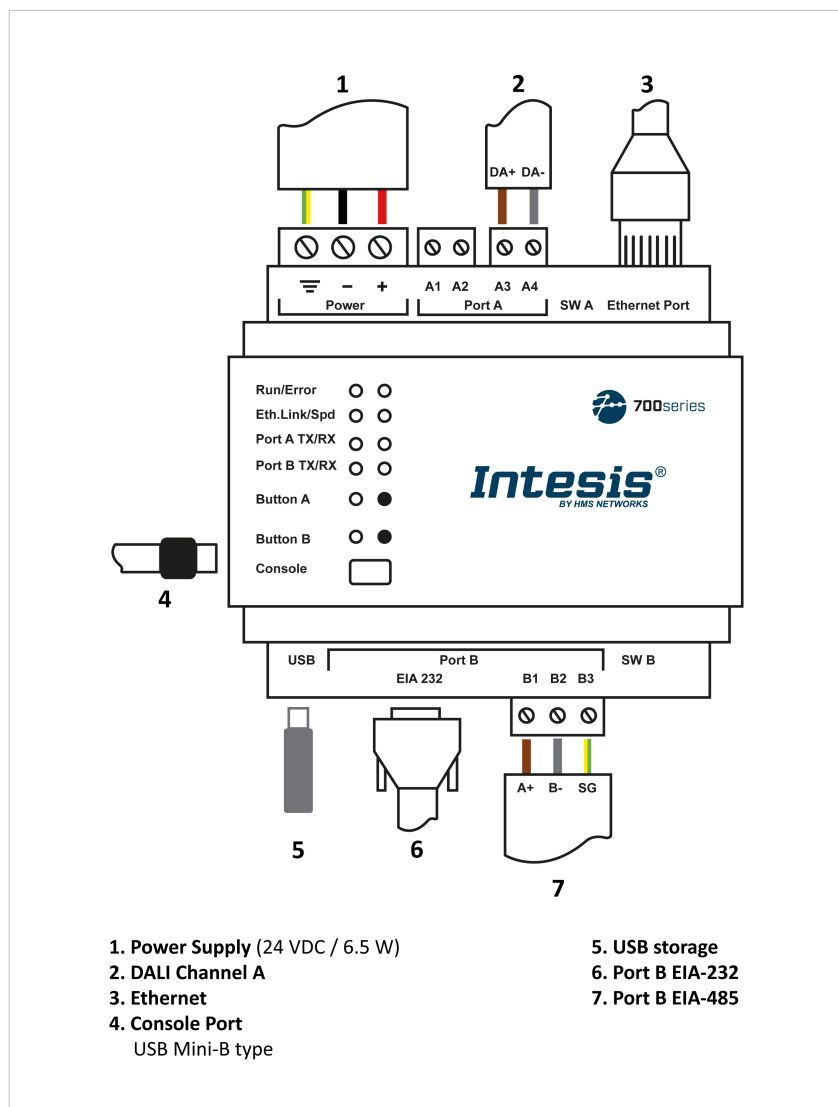
Figure 3. Wiring diagram
