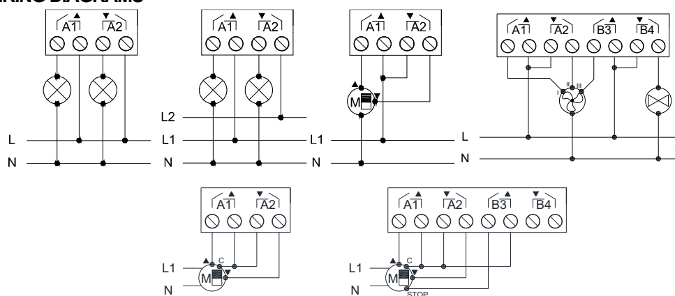
Figure 2: Wiring example (from left to right and up to down): 2 loads, 2 loads connected to different phases, shutter, fan coil, shutter with 2 dry contacts, shutter with 3 dry contacts.
