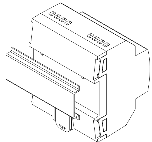
Figure 3: Mounting MAXinBOX 8 v4 on DIN rail
