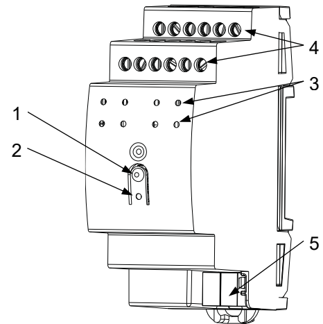
Figure 1: RailQUAD 8 v2
