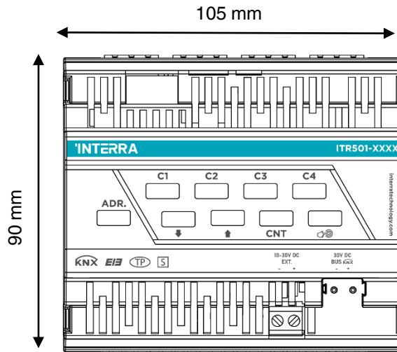
Fig. 2 : Dimension of Universal Dimming Actuator
