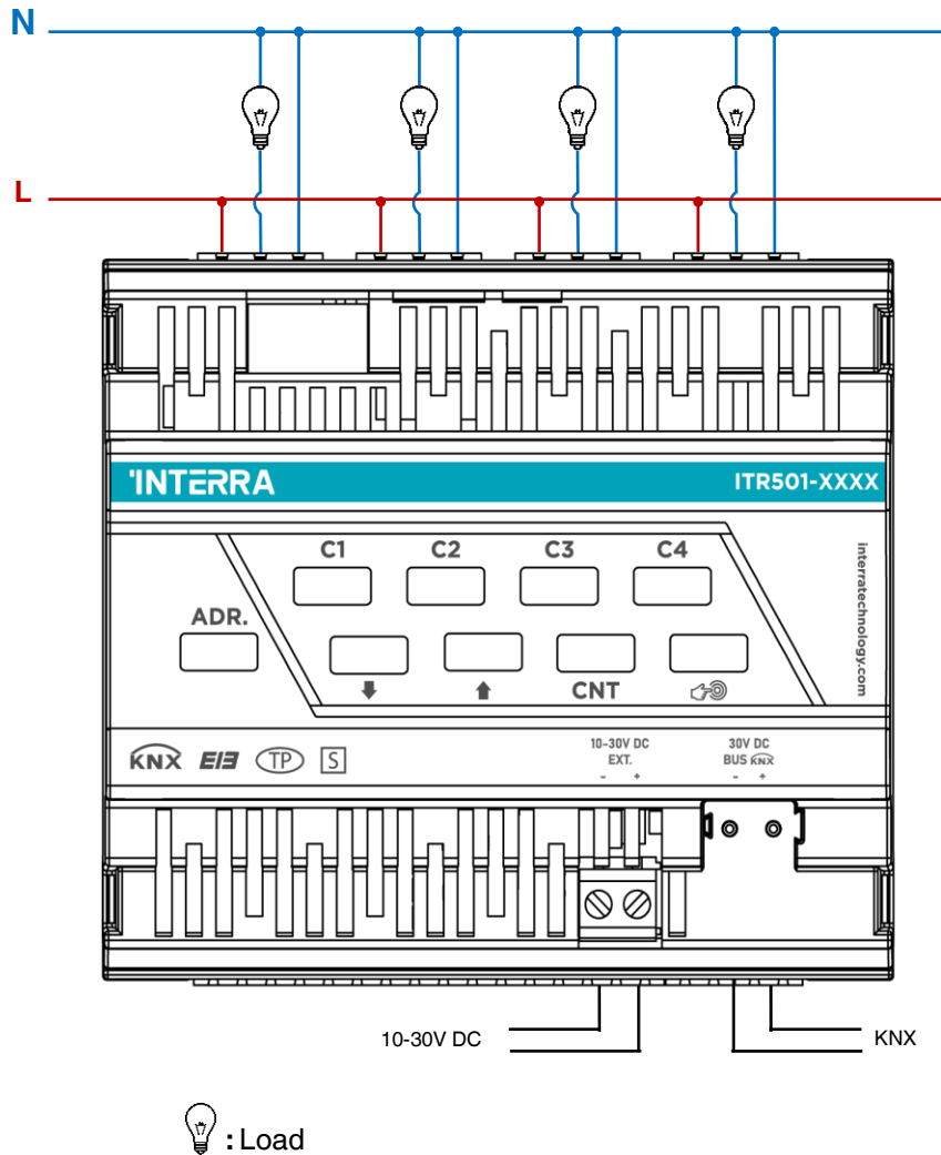
Fig. 1 : Connection Diagram of Universal Dimming Actuator
