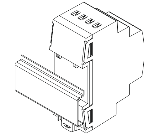
Figure 3: Mounting IndustrialBOX 2 on DIN rail
